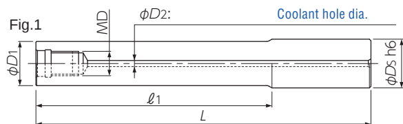
End mill shank type
