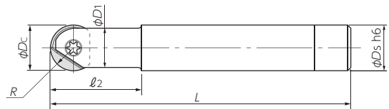
Fig.2 Taper neck
